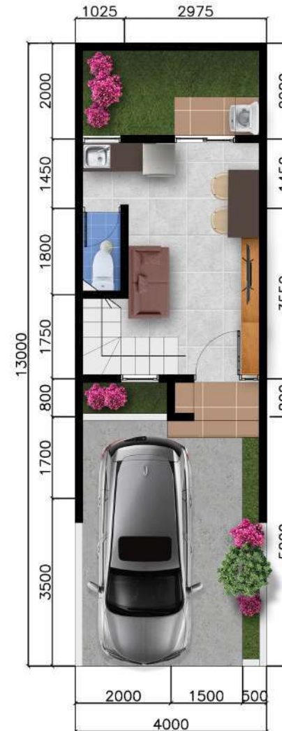
Denah Lantai 1
