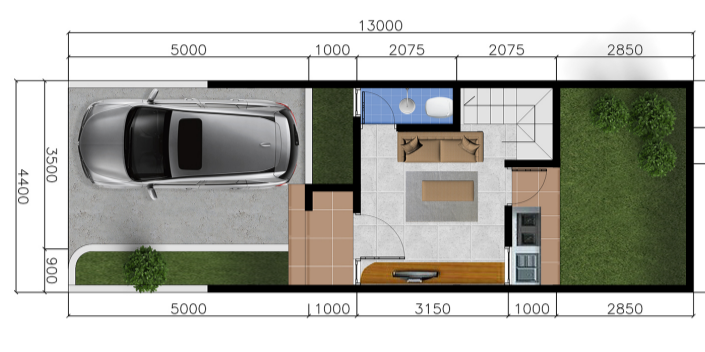
Denah Lantai 1
