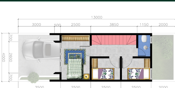
Denah Lantai 2
