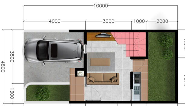
Denah Lantai 1
