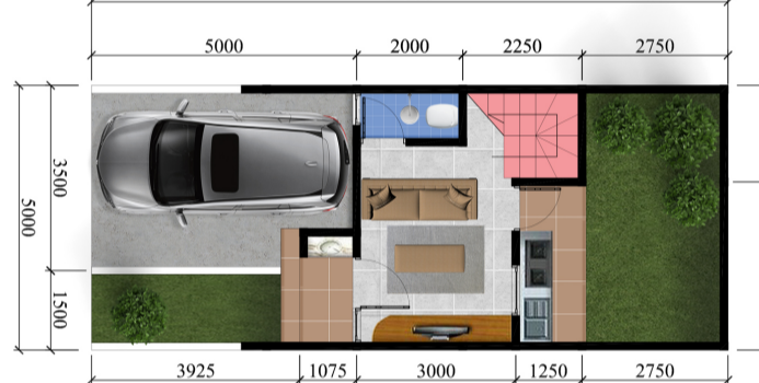
Denah Lantai 1
