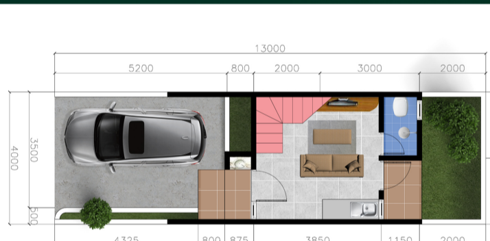
Denah Lantai 1
